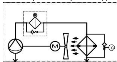
With temperature-dependent bypass valve
