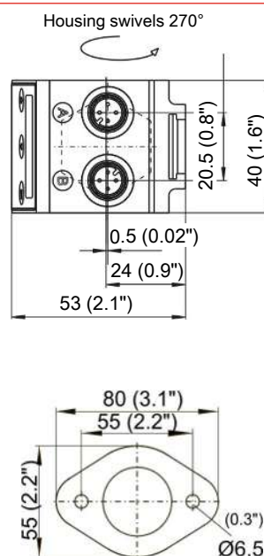
Flange drawing
