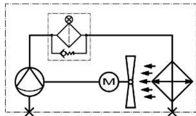
Standard version BNK 2
