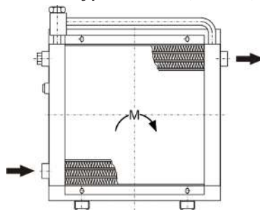
External bypass AB/ATB (BNK 2-6)
