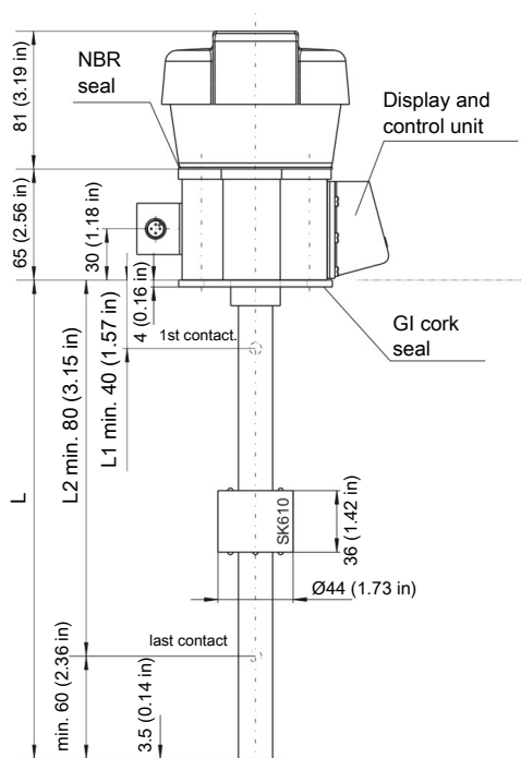
Flange drawing
