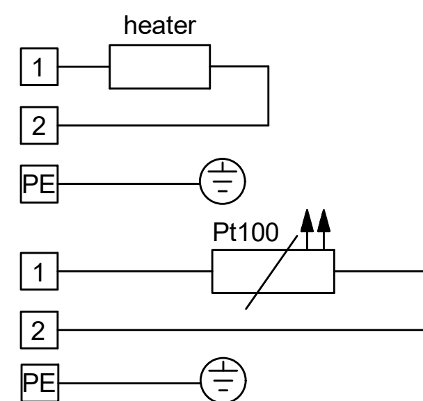
② connecting diagram
